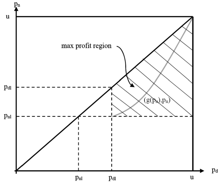
Fig. 1. Equilibrium profits.
